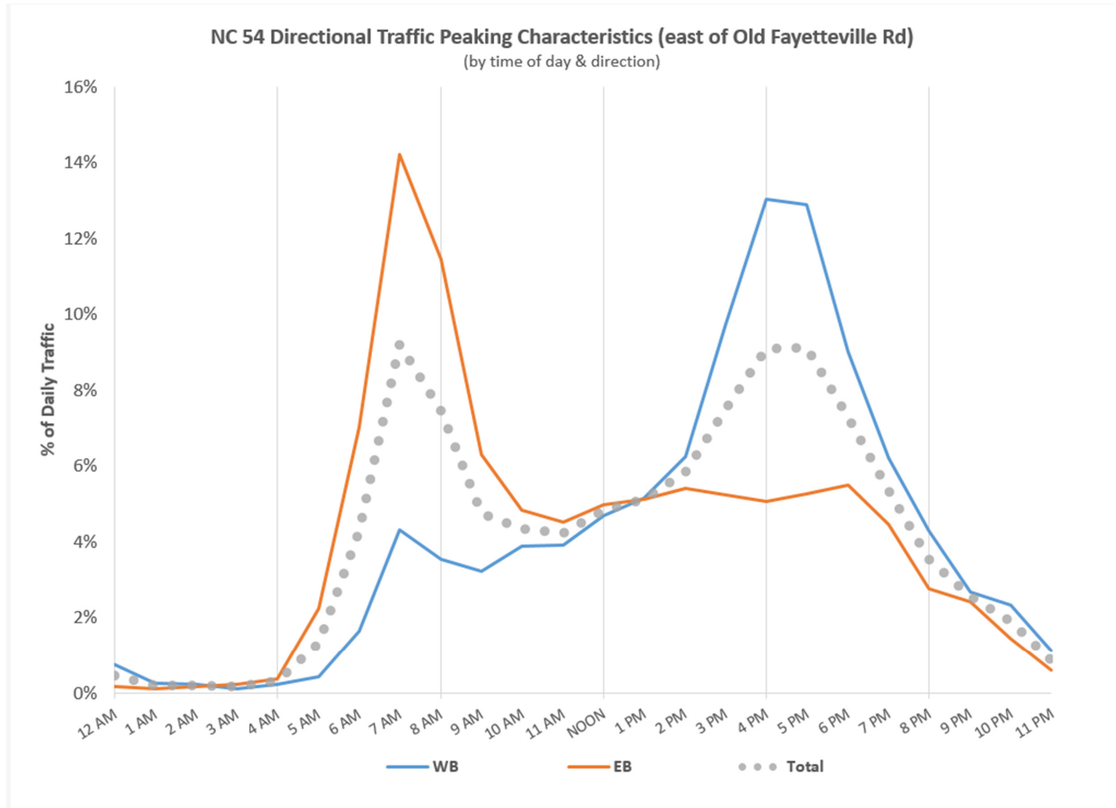
Figure 9: NC 54 Traffic Peaking by Direction (eastern end of corridor)
