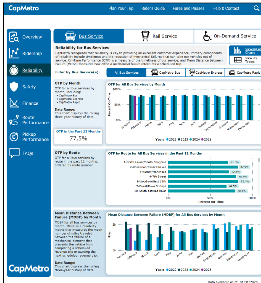
Figure 6-1. CapMetro Dashboard
